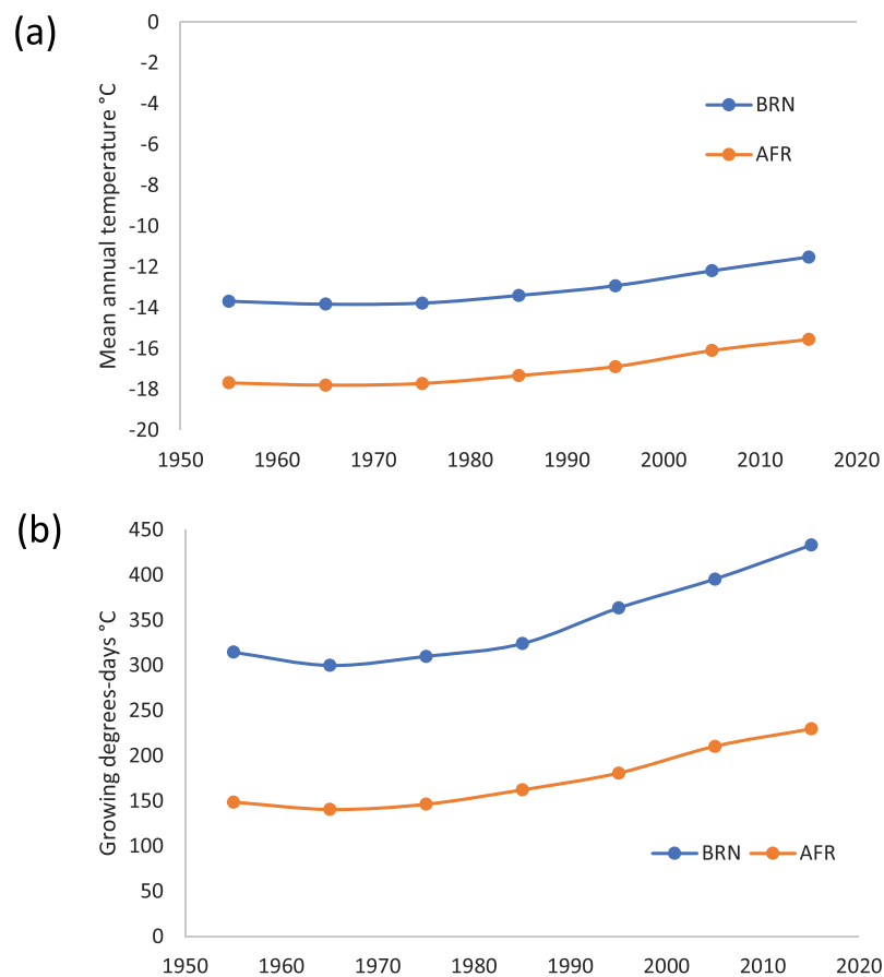
Figure 3. Modeled temperature data showing decadal means for two study sites on Baffin Island: (a) Annual mean temperature and (b) Growing degree days (sum of daily temperatures >0^\circ\text{C} ). Data from ClimateData.ca.
